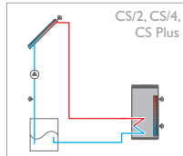
Solar drainback system (Application example)
