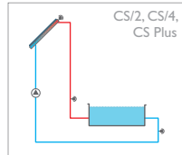
Solar system with swimming pool (Application example)
