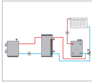
Solid fuel boiler with heating circuit return preheating
