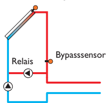
Variante Pumpe:
