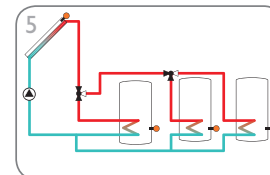
3-store solar system with valve logic and heat exchange control (page 19)
