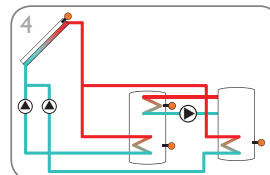
2-store solar system with pump logic and heat exchange control (page 16)
