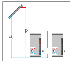
Solar system with 2 stores, 3-port-valve logic
