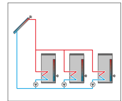
Solar system with 3 stores, pump logic
