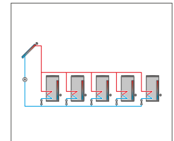
Solar system with 5 stores, valve logic
